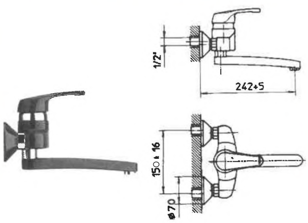
71137 MISCELATORE PARETE MK3 RAP Art. 9210142000 P/C.1
