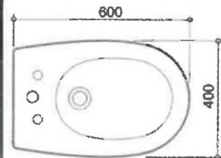
62514 VASO ARETUSA BIAN CSM Art. 72200
