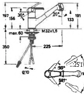
70660 EUROWING MIXLAVELLO C/DOC/E GRO Art. 33809 P/C.1
