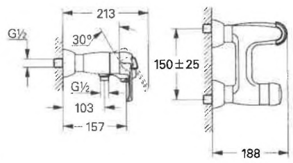
70668 EUROWING VASCA CROMO/ORO GRO Art. 334681G P/C.1
