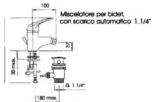
73892 MIX BIDET 1.1/4 SMART CR soi_ Art. 02462R001-CP/C.1
