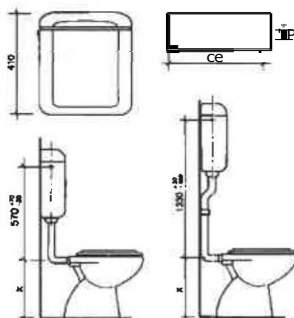
79500 CASSETTA ZAFFIRO .55' 40 BIAN OLV Art. 430201 P/C.5
