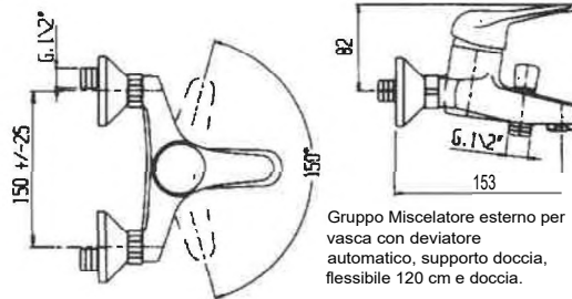
73504 MIX VASCA C/D PUNTA CR SOL Art. 11176-001 P/C.1
