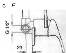
72763 MIX DOCCIA INC VERONA CRO MPB Art. 22032 P/C. 1
