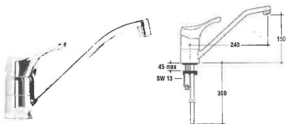
73203 CERAMIX GR LAVELLO IDE Art. A2710AA P/C.1
