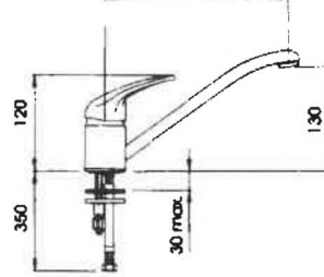
73898 MIKLAVEL MON B/GI SMART C sol Art. 02562R001-CP/C.1
