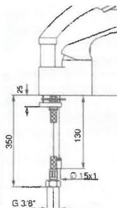
72768 MIXMONPARRUCCH. VERONA MPB Art. 23036 P/C. 1
