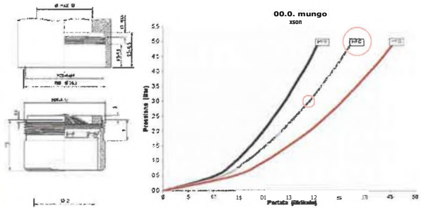
74837 AERATORE x VASCA HFC 28 CR AMF Art. 1051053 PIC.10
