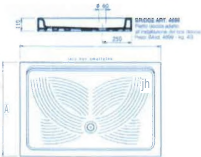
60796 PIATTO BRIDGE 120x80 BIAN DOLArt 4699
