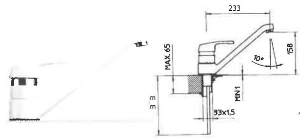
71155 MISC. MONOF LAVELLO MK3 RAP Art. 9401142000 P/C.1
