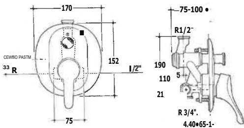
73209 CERAMIX GR INC VASC/D IDE Art. A1993AA P/C.1
