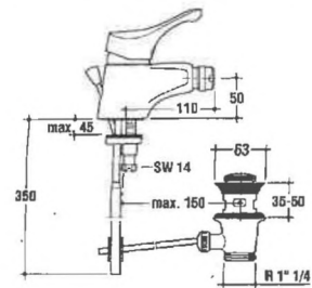
73205 CERAMX GR BIDET IDE Art. A1 182AA P/C.1
