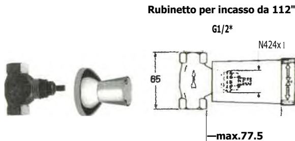
70807 ADRIA RUBINETTO INC. 1/2 GRO Art. 29800+19806 P/C. 1
