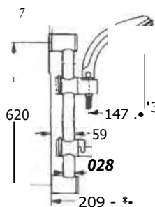
74766 ASTA DOCCIA C/DOC SOFT CR GRO Art. 28646 P/C. 1
