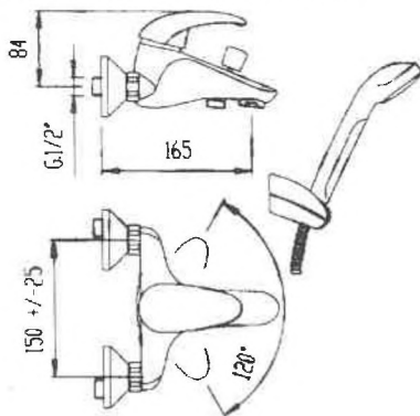
73836 MIX VASCA C/D TALENTO CR SOL Art. 14158.002 P/C.1
