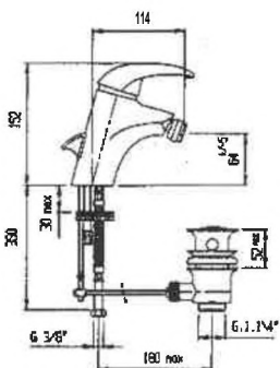
72723 MIX BIDET BARI CRO MPB Art. 3230/E P/C.1
