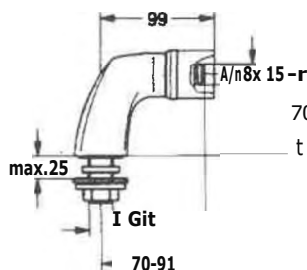
74793 RACCORDO VERTICALE GRO Art. 46121 P/C.1
