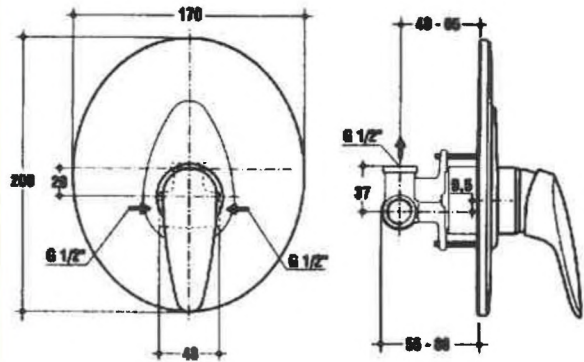
73271 CERAMDC 2000 GR DOCCIA INC IDE Art. A5026AA P/C.
