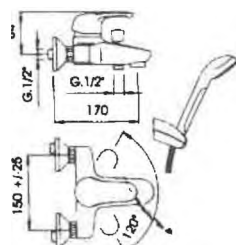
73863 MIX VASCA C/DUPL PRIMA BIA SOL Art. 13168-002NE/P/C.1
