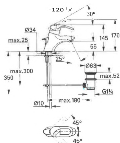
70766 CHIARA MIX LAVABO CROMO GRO Art. 33001 P/C.1
