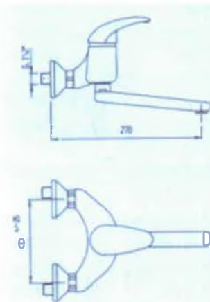
72727 MIX LAVEL.MURO BARI CRO MPB Art. 3630 P/C. 1
