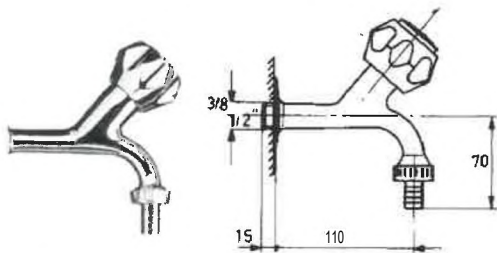
72817 RUBIN:PORT/GOMMA 1/2 MURO RAP Art. 8840000000 P/C.1
