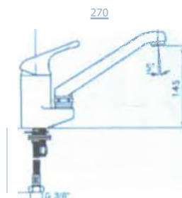
72771 MIXLAV MON B/SPOS VERO CR MPB Art. 25001 P/C. 1
