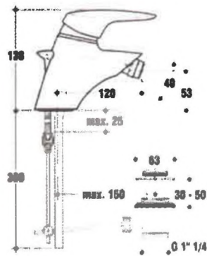
73270 CERAMIX 2000 GR BIDET CR IDE Art. A5016AA
