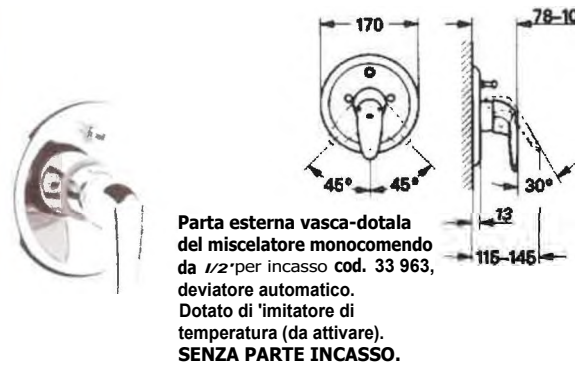
70629 EURODISC ROSONE DOC C/DEV GRO Art. 19548 P/C.
