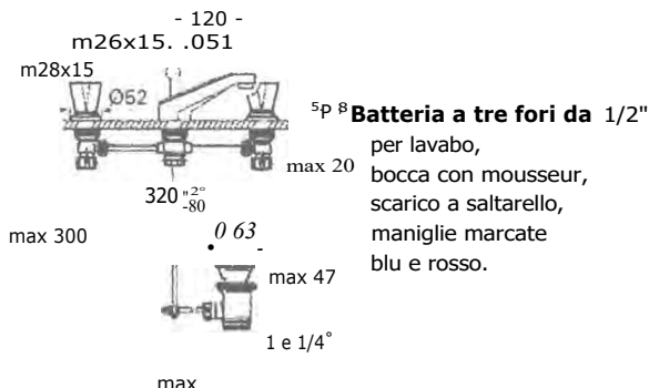
70802 ADRIA BATTERLO LAVABO 3F GRO Art. 20711 P/C.1
