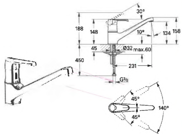
70661 EUROWING MIXLAVELLO GRO Art. 33807 P/C.1
