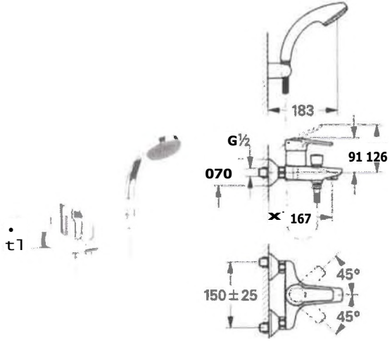
70735 EUROSTYLE MIX VASCA C/D CR GRO Art. 33592 P/C.
