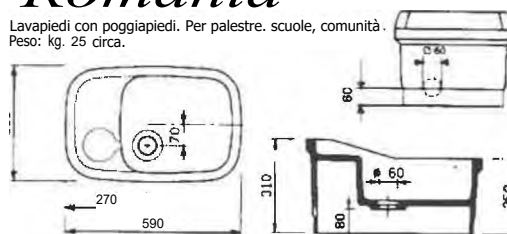
60709 LAVAPIEDI ROMANIA BIAN DOL Art. 4690 P/C.
