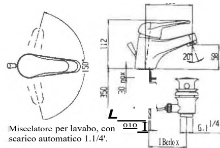
73502 MIX LAVABO PUNTA CR SOL Art. 11376-001 P/C.1
