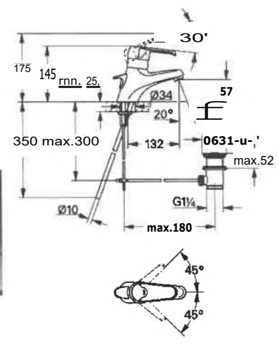
70666 EUROWING LAVABO CR/ORO GRO Art. 330851G P/C.1
