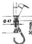
73867 MIX LAV MON D/ES PRIMA BIA SOL Art. 13568-004NE/P/C.1
