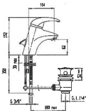
72722 MIX LAVABO BARI CRO MPB Art. 3130/E P/C.1
