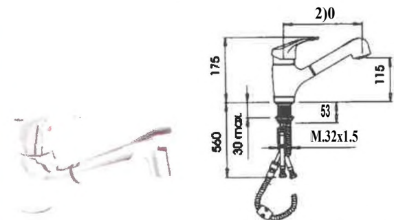
73837 MDC DOCCIA INC TALENTO CR SOL Art. 14258-001 P/C.1
